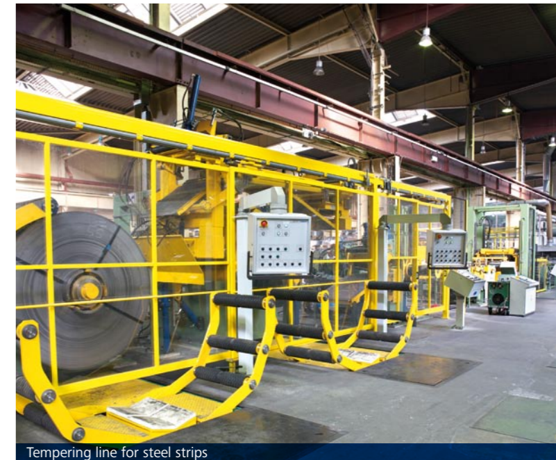
Tempering line for steel strips
